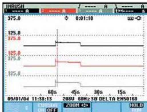
Inrush function automatically triggers off of current, and captures start up measurements on motors and other devices to help determine trip levels.
